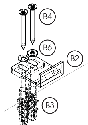
DETAIL C
