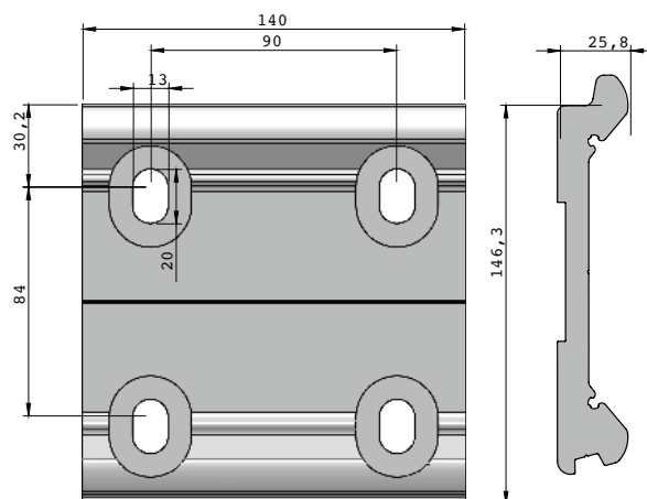
Console murale
