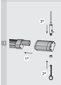
Stainless steel cable Kit self-locking
