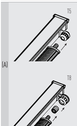
T5 / T8 Replacement
