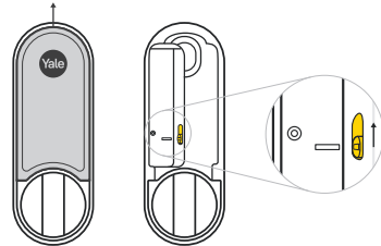
How to remove the battery cover and the mounting plate.
